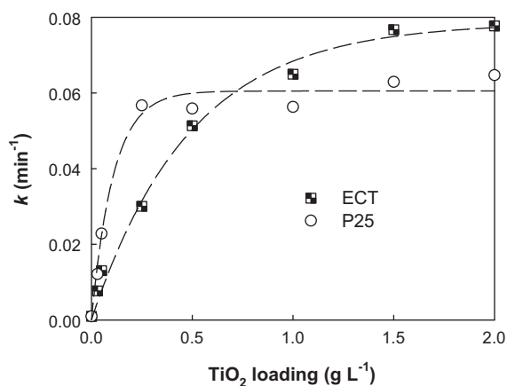
Fig. 1. Pseudo-first order reaction rate constant ( k ) for different catalyst loadings of P25 and ECT photocatalysts at natural pH (5.4).
