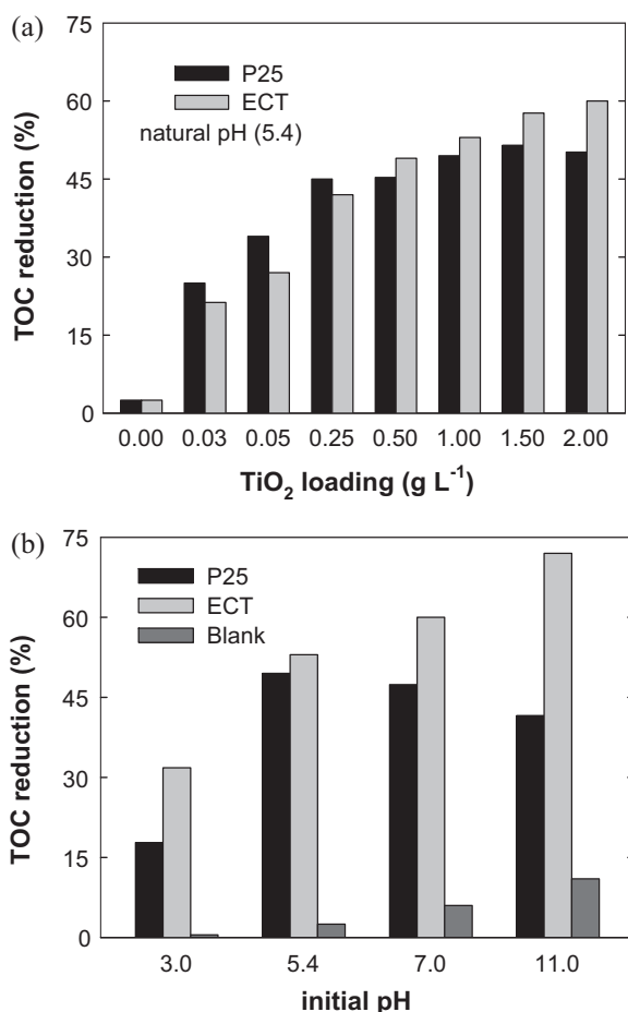
Fig. 3. Total organic carbon (TOC) reduction for different loadings of P25 and ECT photocatalysts at natural solution pH (a) and for different initial solution pH in the presence and absence of 1.00 \text{ g L}^{-1} of P25 and ECT photocatalysts (b).
