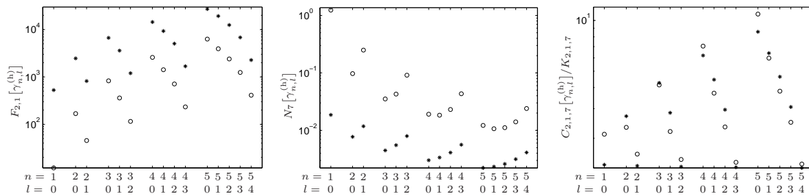
Figure 5. Fisher information F_{p,\beta} (left graph), Rényi entropy power N_\lambda (center graph) and (p, \beta, \lambda) -Fisher-Rényi complexity C_{p,\beta,\lambda} (right graph) of the radial hydrogenic distribution in momentum space with dimensions d = 3(\circ) , 12(*) versus the quantum numbers n and l . The complexity parameters are p = 2, \beta = 1, \lambda = 7 .
