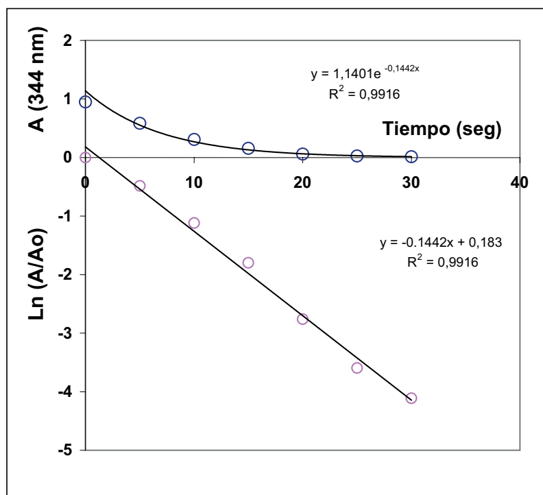
FIGURE 5. Plots of the absorbance measured at 344 nm (upper line) and \ln(A/A_0) vs. time of irradiation at 254 nm of a PDQ solution ( 3.93 \times 10^{-5} M) in ACN.
