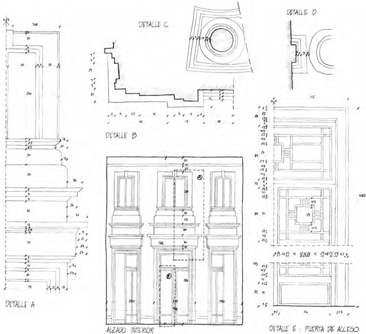
ALZADO INTERIOR
