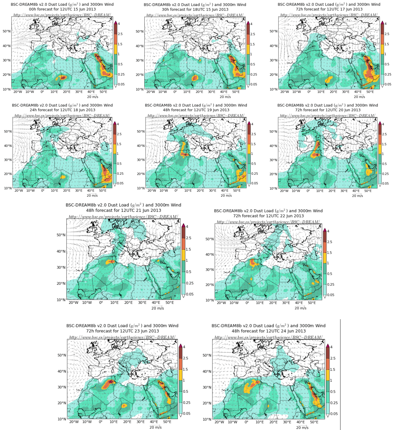
Figure 3. BSC-DREAM8b model images, from 15 to 24 June. The colored areas correspond to the presence of aerosol in the atmosphere.
