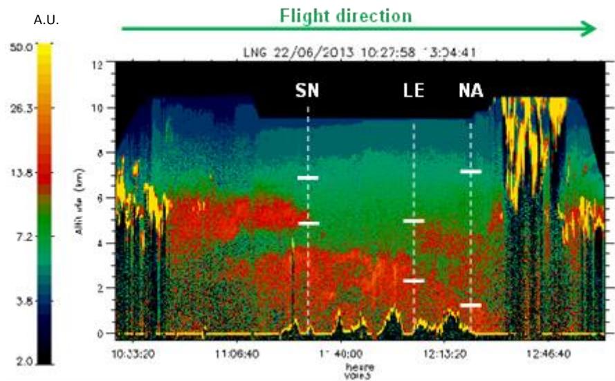
Figure 11. Attenuated backscatter figure of the French Falcon 20 flight on 22 June. The green arrow represents the flight direction. The dash lines are the location of three Italian stations (SN for Serra la Nave, LE for Lecce and NA for Naples), the white lines represents the bottom and top heights of the mineral dust layers detected by the lidars. The red areas correspond to the presence of aerosol.
