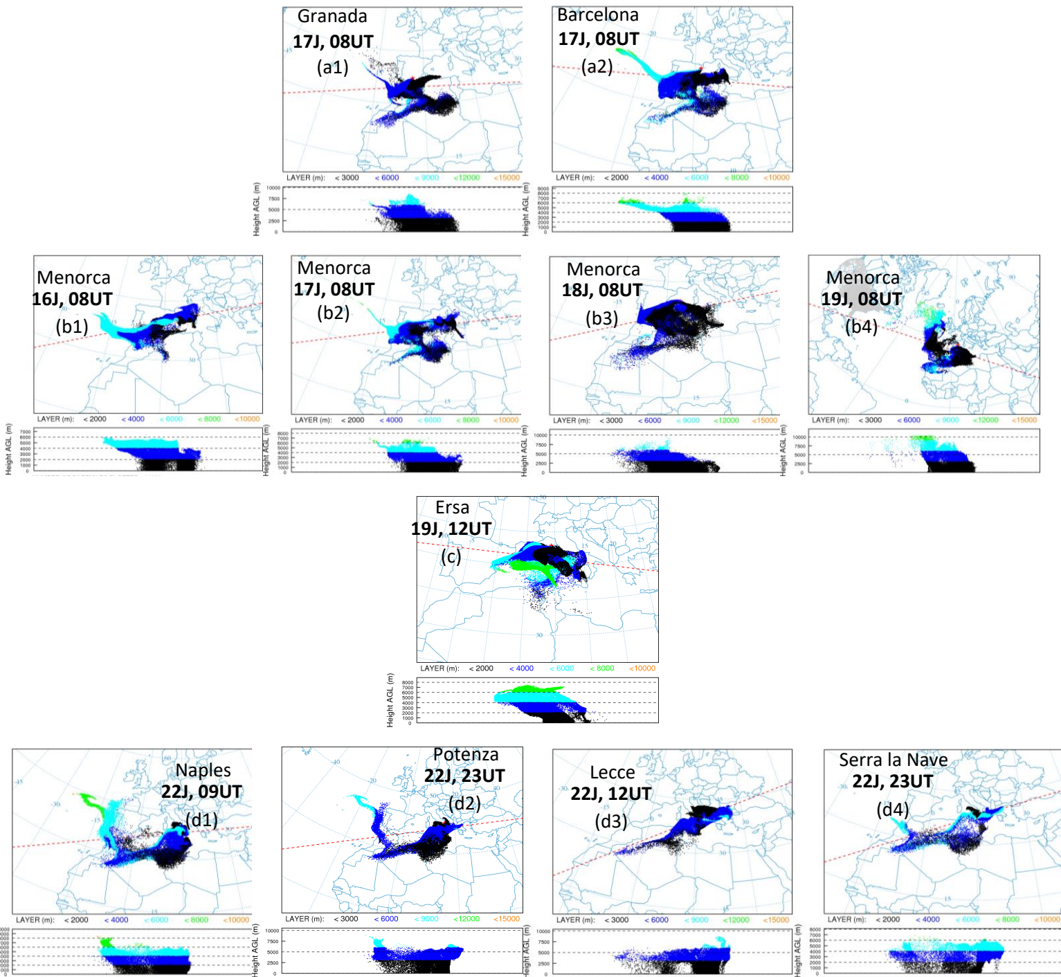
Figure 13. Particle positions simulated during 72 hours with HYSPLIT model. The green areas correspond to the top dust layers, the black areas with the bottom dust layers and the blue (clear and dark) areas with the middle dust layers in each station. 13a) are the particle positions for the Spanish peninsular stations. 13b) are the particle positions for Minorca. 13c) correspond to the particle positions in Ersa, and 13d) are the particle positions simulated for the Italian stations. In the plots located in the lower part, the X axis indicates time and the Y axis indicates height AGL (m).
