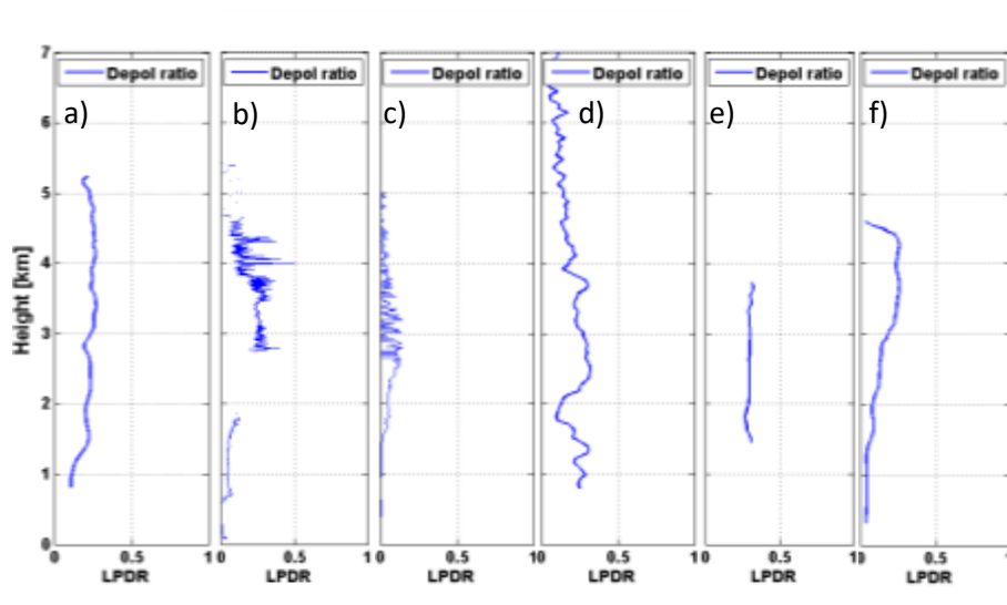
Figure 7. Particle depolarization ratios retrieved by lidar measurements. From the left to the right the stations are Granada at 532 nm (a), Minorca at 355 nm (b), Ersa at 355 nm (c), Naples at 532 nm (d), Potenza at 532 nm (e), Lecce at 355 nm (f). The date of the measurements are 17 June at 01 UTC, 18 June at 12 UTC, 20 June at 15 UTC, 22 June at 10:46 UTC, 21 June at 23:40 and 22 June at 11:18 for Granada, Minorca, Ersa, Naples, Potenza and Lecce respectively. The bottom and top heights are 2236 and 5994 m in Granada, 201 and 5787 m in Minorca, 1360 and 4848 m in Ersa, 1768 and 7468 m in Naples, 1630 and 5530 m in Potenza and 1484 and 5081 m in Lecce.
