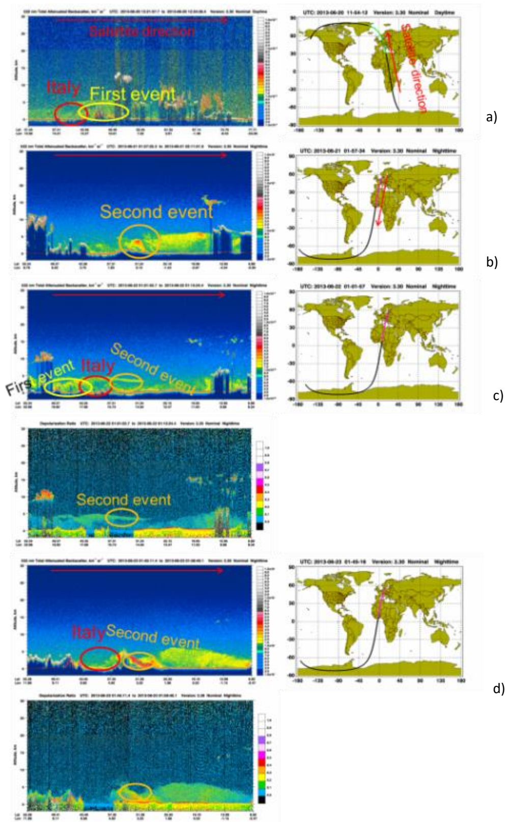
Figure 10. Spatio-temporal evolution of the dust plume monitored by CALIPSO overpasses. In red Italy, in yellow the first Saharan dust event and in orange the second Saharan dust event. a) Attenuated backscatter figure of the day time overpass of the 20 June. b) Attenuated backscatter figure of the night time overpass of the 21 June. c) Attenuated backscatter and lidar particle depolarization ratio figures of the night time overpass of the 22 June. d) Attenuated backscatter and lidar particle depolarization ratio figures of the night time overpass of the 23 June.
