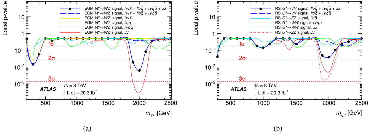
Fig. 2. The p_0 -value for the individual and combined channels for (a) the EGM W' search in the \ell\nu\ell'\ell' , llq\bar{q} , lvq\bar{q} and JJ channels and (b) the bulk G^* search in the llq\bar{q} , lvq\bar{q} and JJ channels.
