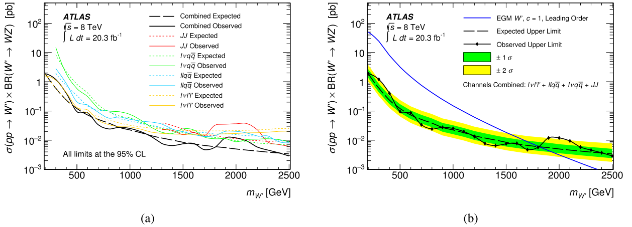
Fig. 3. The 95% CL limits on (a) the EGM W' using the \ell\nu\ell'\ell' , llq\bar{q} , lvq\bar{q} , and JJ channels and their combination, and (b) the combined 95% CL limit with the green (yellow) bands representing the 1\sigma ( 2\sigma ) intervals of the expected limit including statistical and systematic uncertainties. (For interpretation of the references to colour in this figure legend, the reader is referred to the web version of this article.)
