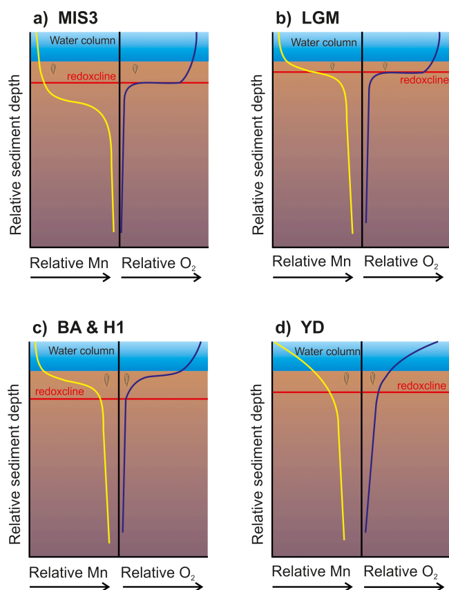
Figure 5. Idealised schematic pore-water Mn (yellow) and oxygen (blue) profiles for the climatic intervals studied from the GeoB7926-2 record. The red line represents the redoxcline. (a) MIS3: low foraminiferal Mn / Ca, and therefore the sedimentary Mn was precipitating below the living depth of E. exilis and more-oxygenated conditions prevailed in the bottom and pore waters. (b) LGM: foraminiferal Mn / Ca increases, and therefore a relative decrease in pore-water oxygen is apparent and the redoxcline is shallower. (c) BA & H1: foraminiferal Mn / Ca increases further, and the moderate–low sedimentary Mn / Al indicates low bottom-water conditions. (d) YD: highest accumulation of Mn and therefore oxygen deficiency in the bottom and pore waters.
