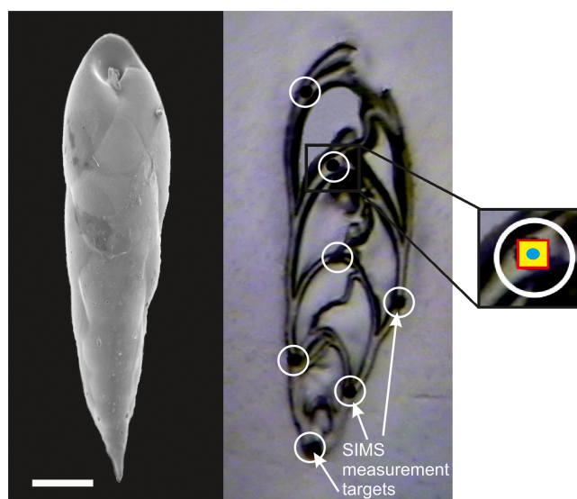
Figure 2. SEM image (scale bar: 100\ \mu\text{m} ) and cross-section image during SIMS analysis of a single Eubuliminella exilis specimen. The white circles highlight the selected spots for SIMS analyses, measuring 5\ \mu\text{m} in diameter. Note that the black areas of the SIMS measurement targets visible in this image are actually the 5\ \mu\text{m} spots plus the 10\ \mu\text{m} pre-sputters. Inset is a close-up of the SIMS targets: the red square is the approximate pre-sputter area ( 15 \times 15\ \mu\text{m} , i.e. 5\ \mu\text{m} spot + 10\ \mu\text{m} raster), the yellow area is the field of view admitted to the mass spectrometer (controlled by magnification and field aperture) and the blue ellipse is the nominal 5\ \mu\text{m} spot.
