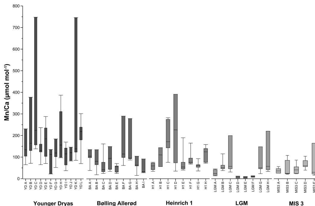
Figure 3. The Mn / Ca ( \mu\text{mol mol}^{-1} ) variability within each individual Eubulimina exilis specimen for each climatic interval (labelled on the x axis), determined by SIMS.
