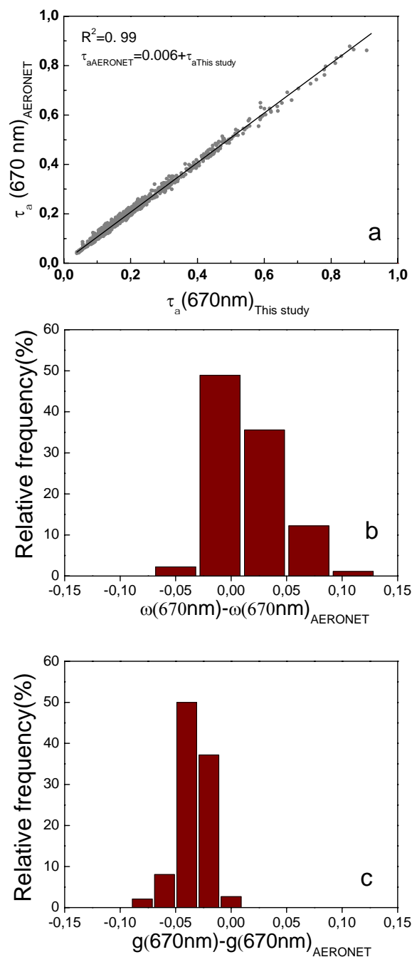
Fig. 2. (a) \tau_a(670\text{nm}) provided by AERONET vs the data computed by our methodology. (b) and (c) Frequency distributions of the absolute differences between \omega(670\text{nm}) and g(670\text{nm}) provided by AERONET and computed by the Principal plane inversion algorithm.
