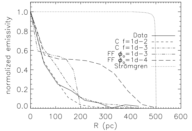
Fig. 3. Observationally derived H \alpha radial emissivity profile of a bright H II region of the barred spiral galaxy NGC 1530 (solid line). The profile has been normalized to facilitate its comparison with the profiles predicted by clumpy and FF models. The spatial resolution of the four theoretical models has been degraded to match the resolution of the H \alpha image of NGC 1530 (approx. 50 pc per pixel). We can see that the clumpy models produce concave profiles, similar to the observations. On the contrary, FF models, give rise to convex profiles. The dotted line represents an ideal Strömgen model, whose ionization fraction is constant and equal to 1 inside the H II region volume, except close to the boundary of the Strömgen sphere.
