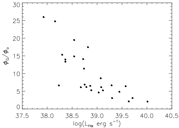
Fig. 7. Ratio between the geometrical and optical filling factors as a function of H\alpha luminosity for H II regions from the catalogue of NGC 1530 (Relaño et al. 2004). \phi_G has been obtained assuming spherical clumps with radius 1 pc and a photon escape fraction of 30%. Under this hypothesis, the mean ratio of filling factors is \sim 10 , while assuming a photon escape fraction of 50% the mean ratio is \sim 6 .
