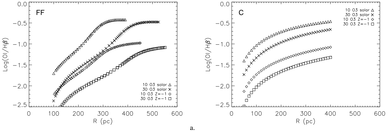
Fig. 6. a.) Behaviour of line ratio [\text{O I]6300}/\text{H}\beta versus the H II region radius for different families of H II region models in the FF approximation, for two different stellar contents and metallicities. As the radius increases, the regions change from density to ionization bounded. The [\text{O I]6300}/\text{H}\beta ratio becomes constant when the models become ionization bounded. b.) Same as a.) but for clumpy models. In this case the line ratio increases very slowly because the emission lines result from the sum of the contribution of all the clumps, which are ionization bounded. The reason why we see a slow increase rather than a plateau is due to the fact that each clump has a different ionization parameter, depending on its distance from the ionizing stellar source.
