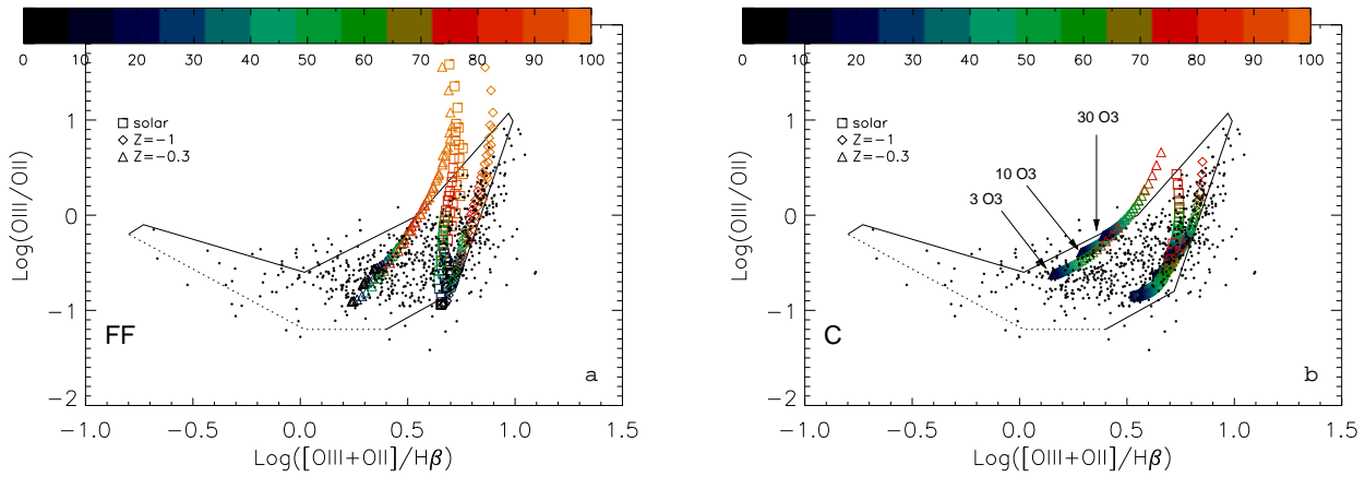
Fig. 4. Density bounding diagnostic diagram (McCall et al. 1985). Solid lines delimit the area occupied by McCall’s data and the dotted line indicates where this limit is least certain. Data points correspond to H II region observations, which have been obtained from Cedrés & Cepa (2002), Van Zee et al. (1998), Kennicutt & Garnett (1996), Walsh & Roy (1997) and Roy & Walsh (1997). Colour symbols refer to models (FF in a. and clumpy in b. ) assuming 3, 10 and 30 ionizing O3 type stars and 3 different abundances: 0.1 solar, 0.5 solar, and solar. Colours indicate the escape fraction of ionizing photons in each case. We can see that all models, even those with a strong escape fraction, are located in the areas covered by the observational data.
