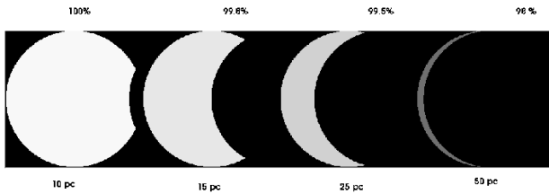
Fig. 1. Equatorial section of a spherical clump with density 100 \text{ cm}^{-3} and radius 1 \text{ pc} illuminated by an ionizing source and placed at different distances from it. The light area represents the ionized volume of the clump (seen in cross-section) and the dark area represents the volume which remains neutral. Gray areas show partial ionization. In this example, obtained with CLOUDY, we used an ionizing source emitting 10^{42} \text{ erg s}^{-1} yielding conservatively high clump ionization.
