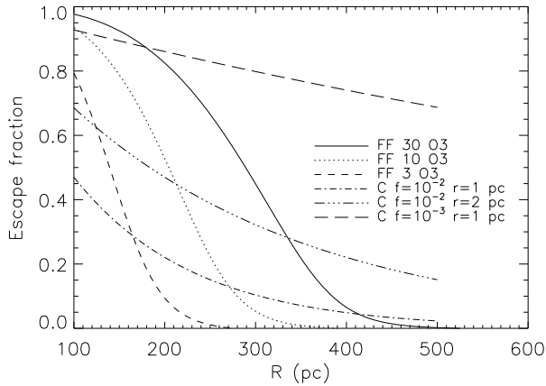
Fig. 2. Dependence of photon escape fraction on the H II region radius for different models. In classical FF models, the escape fraction depends on the radius, on the filling factor, and on the strength of the ionizing radiation (we have considered ionizing clusters with 3, 10, and 30 O3 type stars, and a filling factor of 10^{-4} ). In contrast, in the clumpy models the dependence is only geometrical; in other words, the escape fraction depends on the radius of the region, and on the radius and density of the clumps. We show results of three clumpy models (labeled with C) assuming different filling factors 10^{-2} , 10^{-3} and clump radii (1 and 2 pc).
