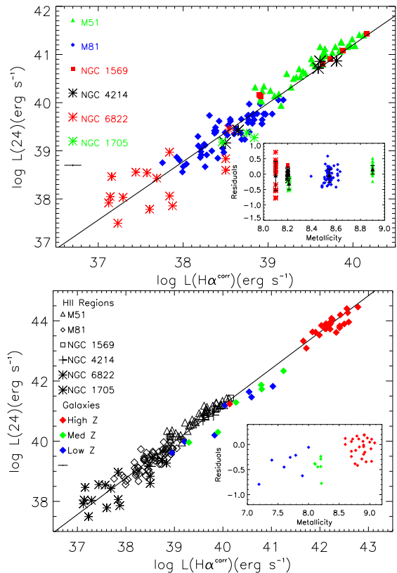
FIG. 1.— Top : 24\mu\text{m} luminosity as a function of the extinction corrected \text{H}\alpha luminosity for a sample of \text{H II} regions in M51, M81, NGC 1569, NGC 4214, NGC 6822 and NGC 1705. The solid line shows the linear fit to the \text{H II} regions of M51, M81 and the ULIRGs from Alonso-Herrero et al. (2006) (see Eq. 1). Typical error bars are shown in the lower left corner of the plot: they account for uncertainties in the calibration (4% for 24\mu\text{m} flux (Engelbracht et al. 2007), \sim 15\% for \text{H}\alpha flux and \sim 0.2\text{mag} for the extinctions (Gil de Paz et al. 2003; Relaño et al. 2006)). In the inner panel we show the residuals of the 24\mu\text{m} luminosity (see text) versus the metallicity. The black triangles represent the mean value of the residuals for each galaxy. Bottom : The same plot as above but including the integrated luminosities of the galaxies in Table 1. The solid line is the linear fit shown in Eq. 1. We use different colors for galaxies with different metallicities: Z \leq 8.0 (blue), 8.0 < Z < 8.5 (green) and Z \geq 8.5 (red). In the inner panel we show the residuals of the 24\mu\text{m} luminosity with respect to linear fit (Eq. 1) versus the metallicity.
