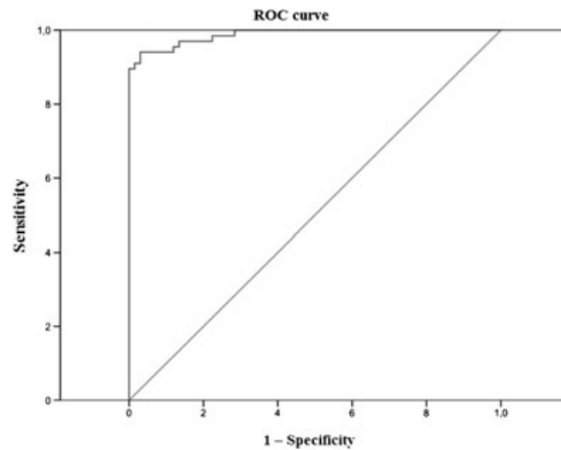
Figure 1. ROC curve model of multivariate analysis of emerging and classic cardiovascular risk factors for acute coronary syndrome.
