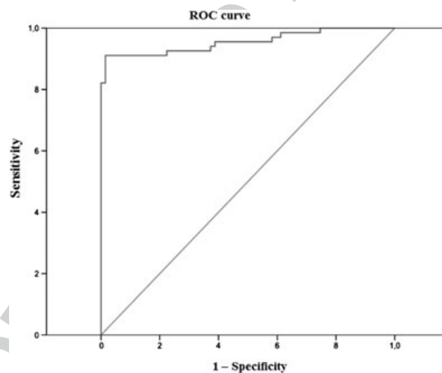
Figure 2. ROC curve model of multivariate analysis of emerging and classic cardiovascular risk factors for stroke.
